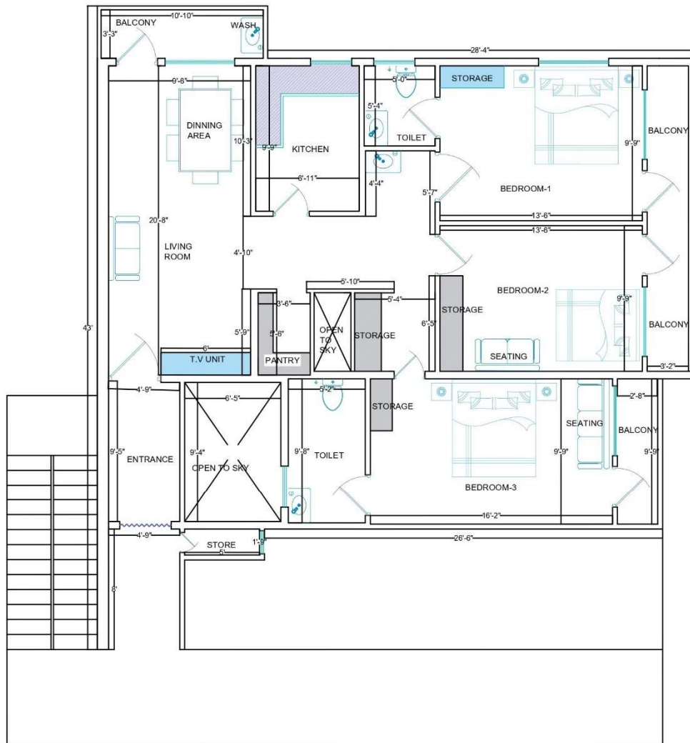
LAYOUT PLAN FOR INDIAN BANK GUEST HOUSE
