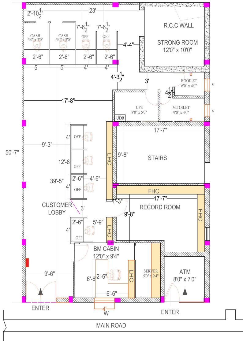
FINAL DRAWING
