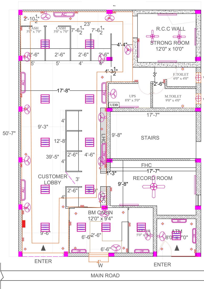
EXISTING GROUND FLOOR PLAN ELECTRICAL LAYOUT
