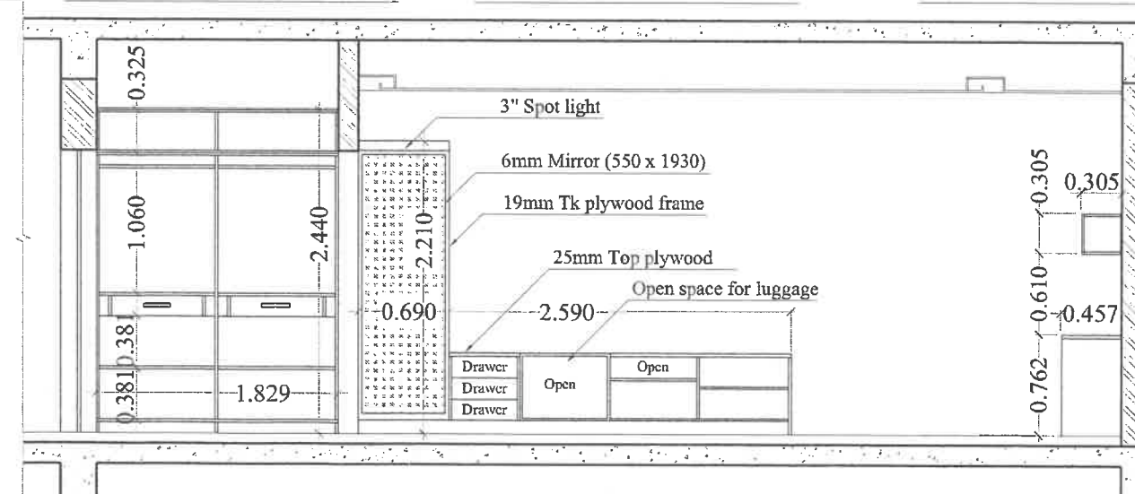
INTERNAL ELEVATION
