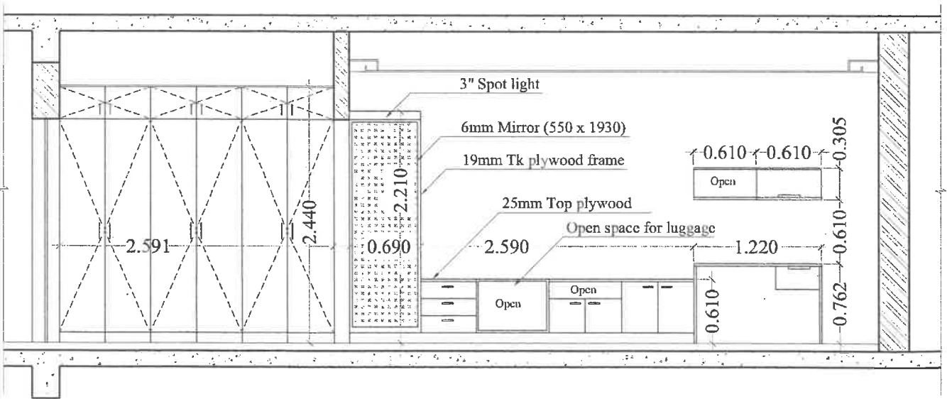
EXTERNAL ELEVATION
