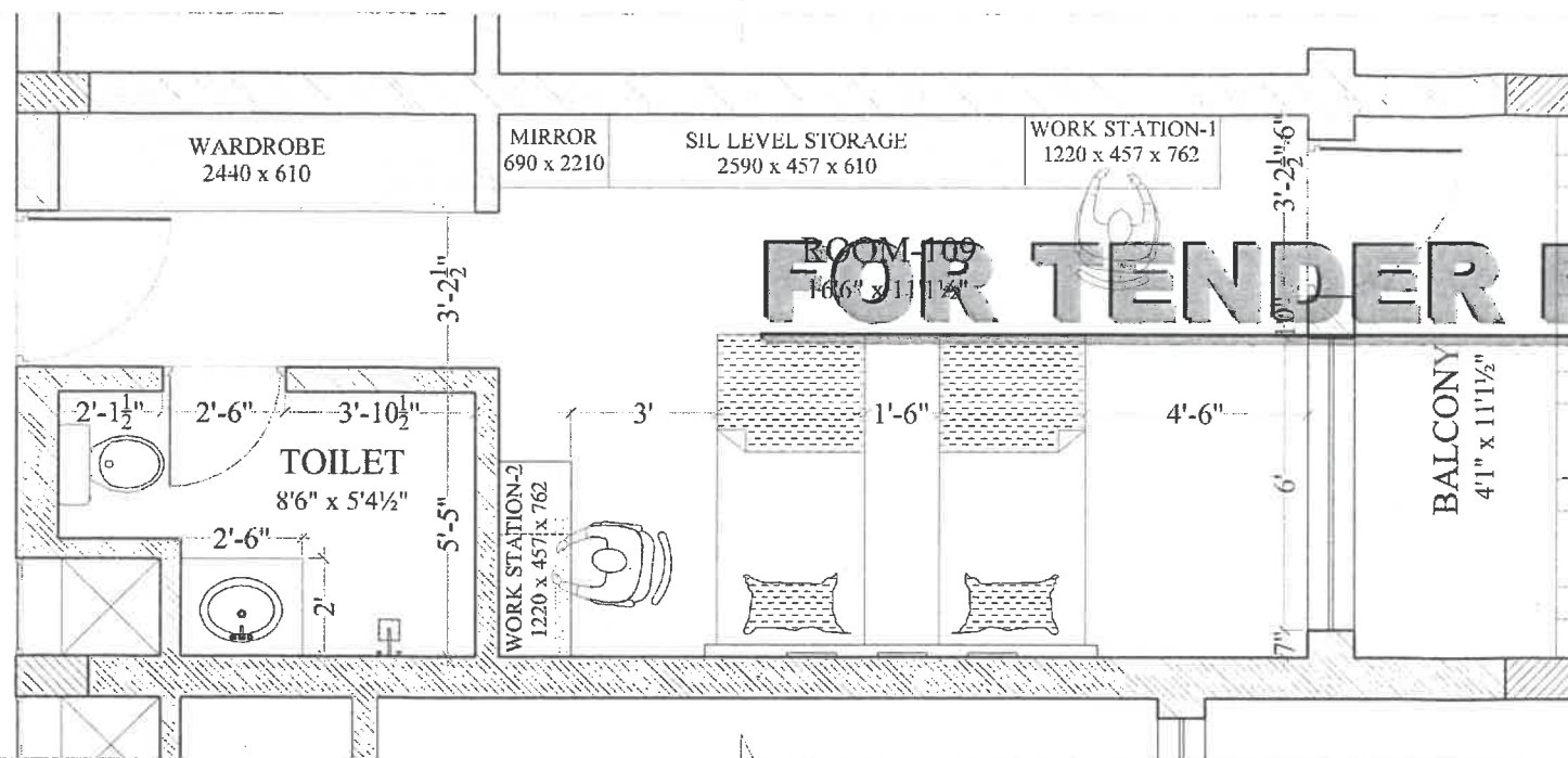
PLAN OF ROOM -109
