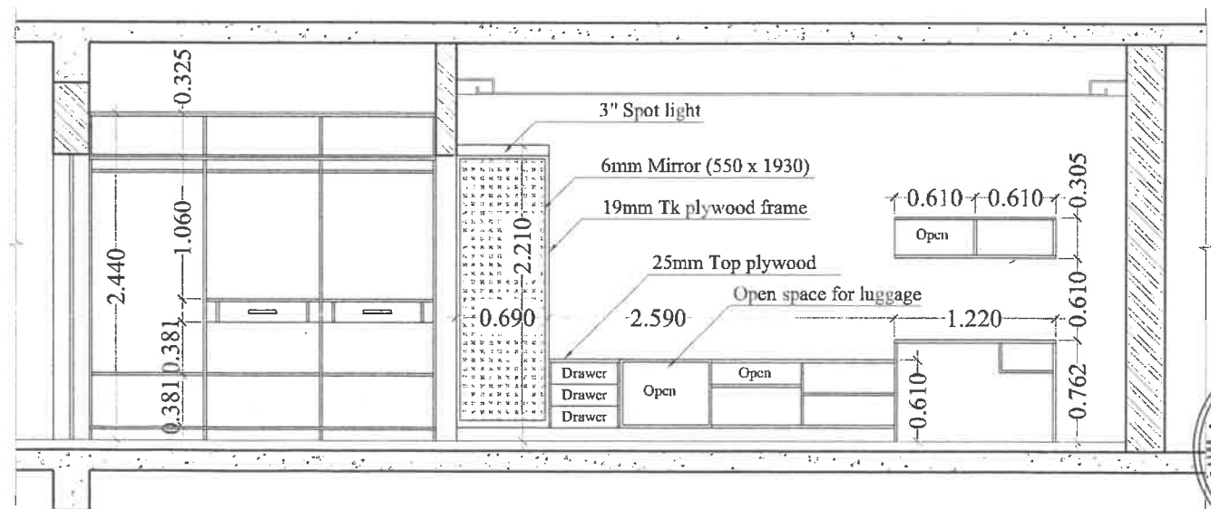
INTERNAL ELEVATION
