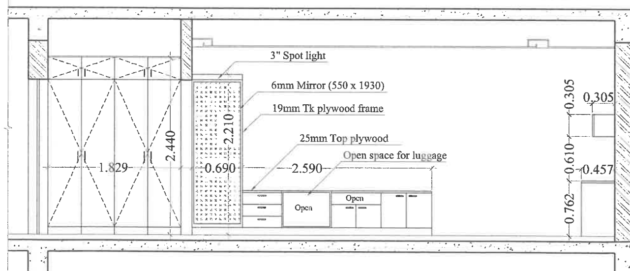
EXTERNAL ELEVATION
