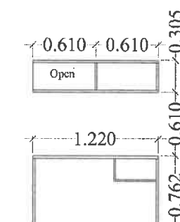
INTERNAL ELEVATION
