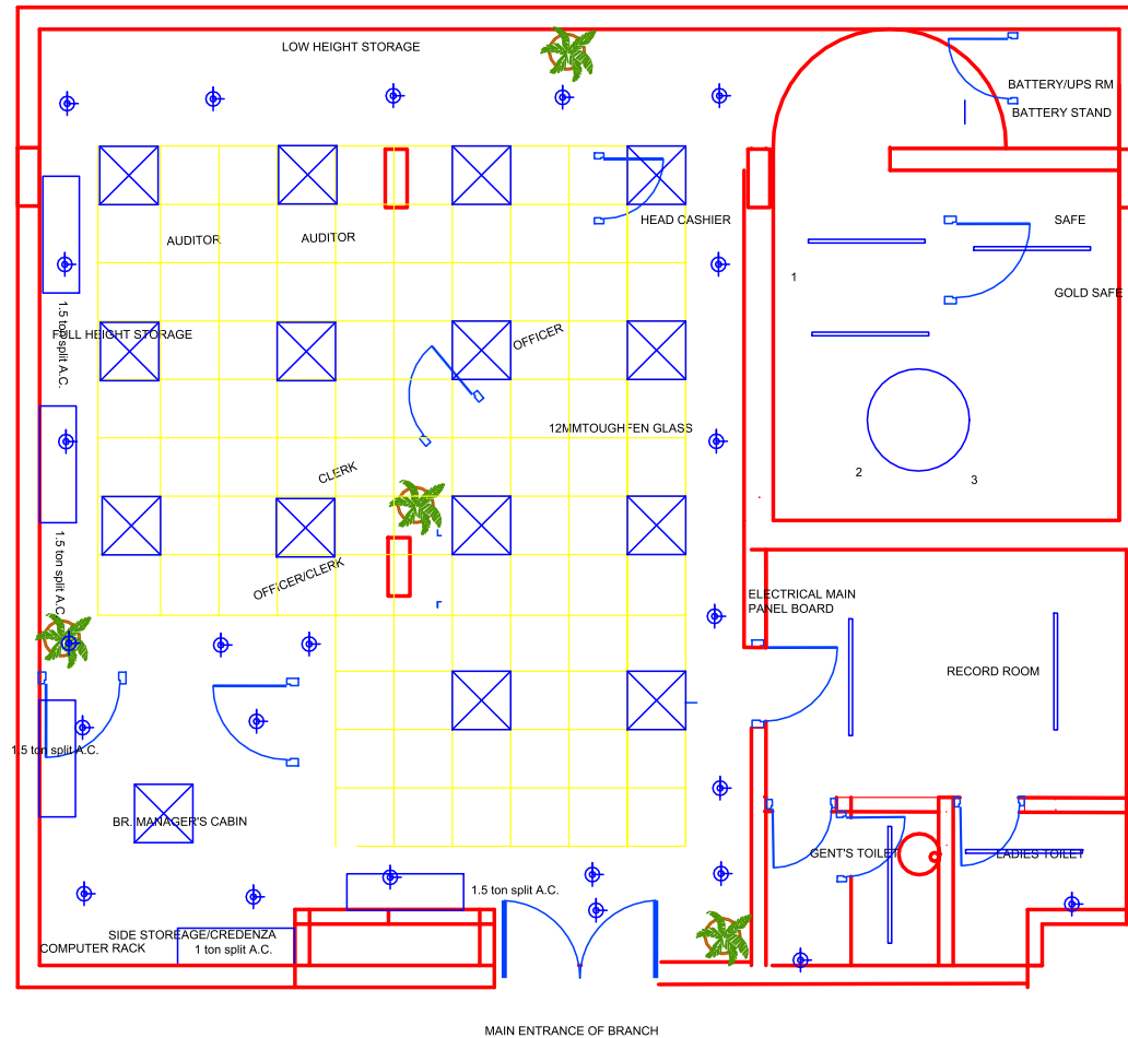
PROPOSED ELECTRICAL LAYOUT
