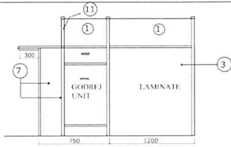
SECTION @ X
