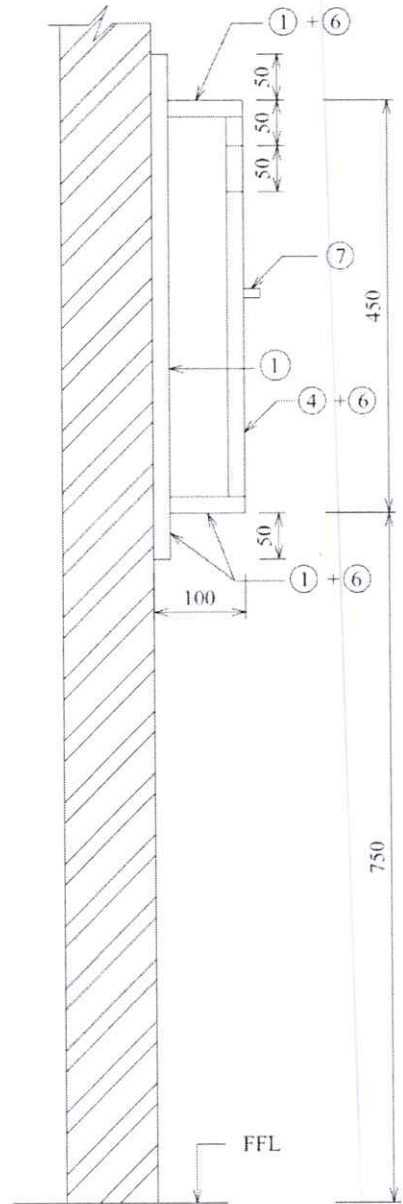
SECTION@DD
