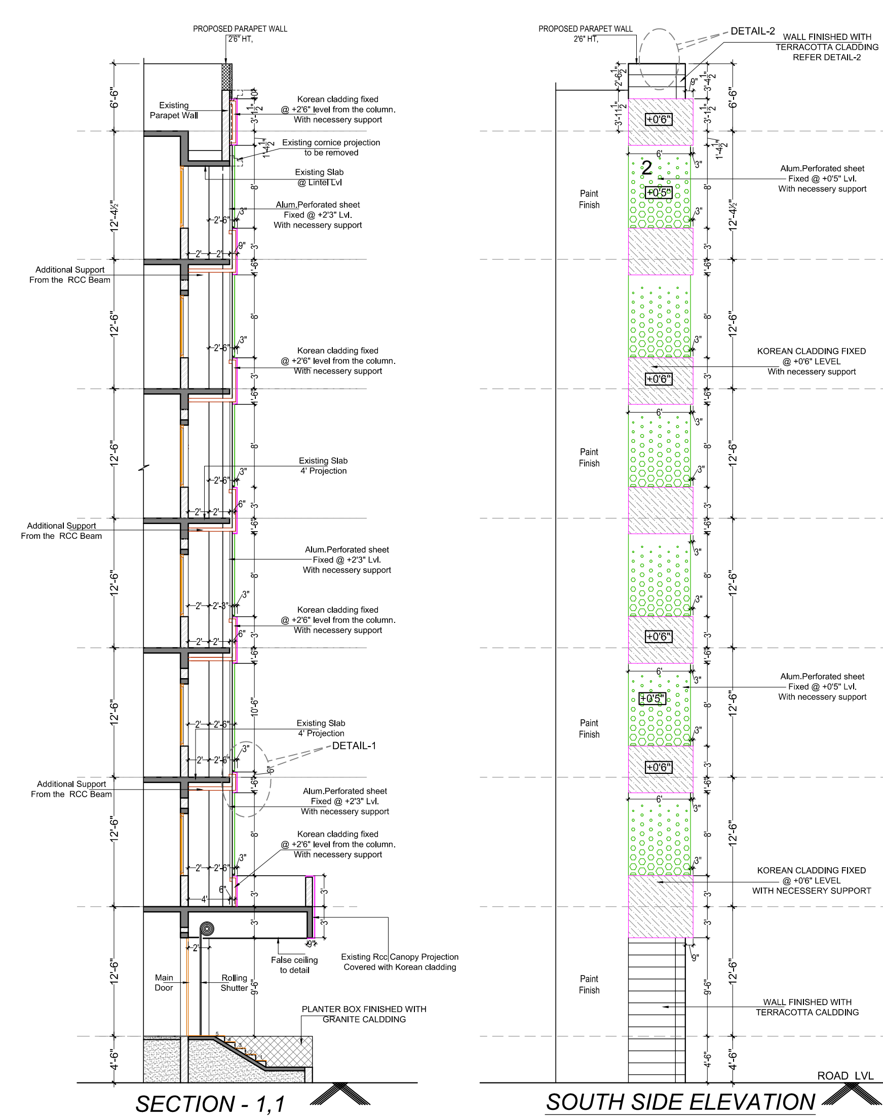
SOUTH SIDE ELEVATION
