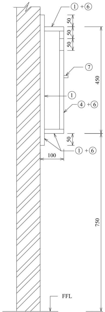
SECTION@DD
