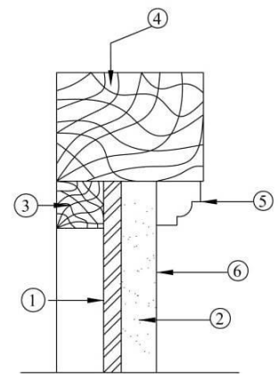
DETAIL AT 'Z'
