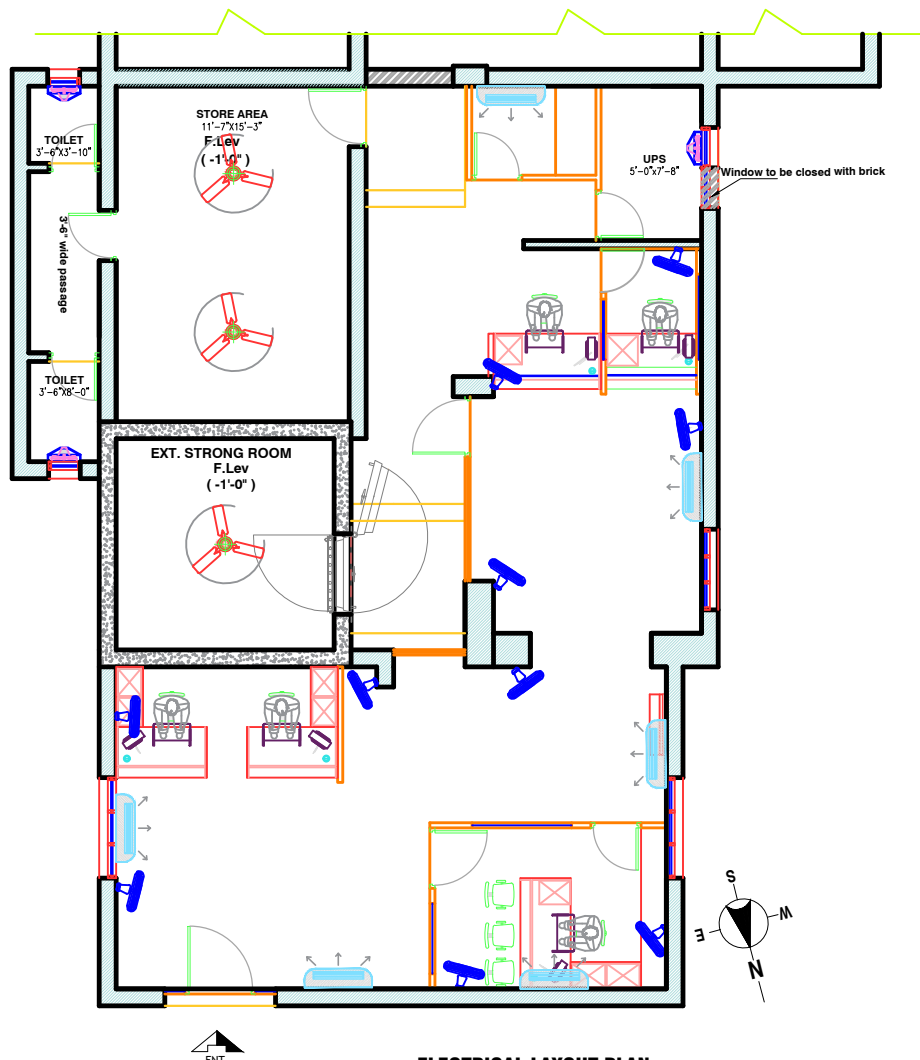
ELECTRICAL LAYOUT PLAN
