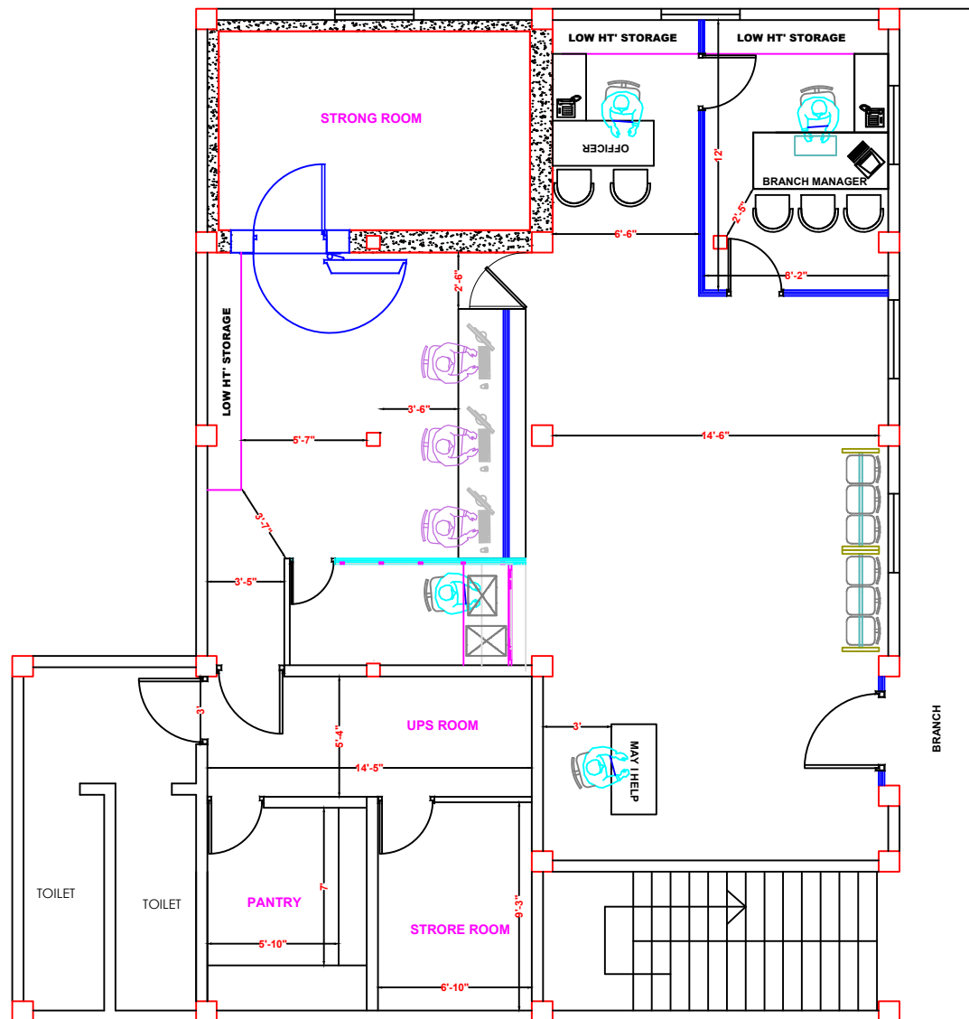
PROPOSED LAYOUT PLAN FOR GHORMARA BRANCH
